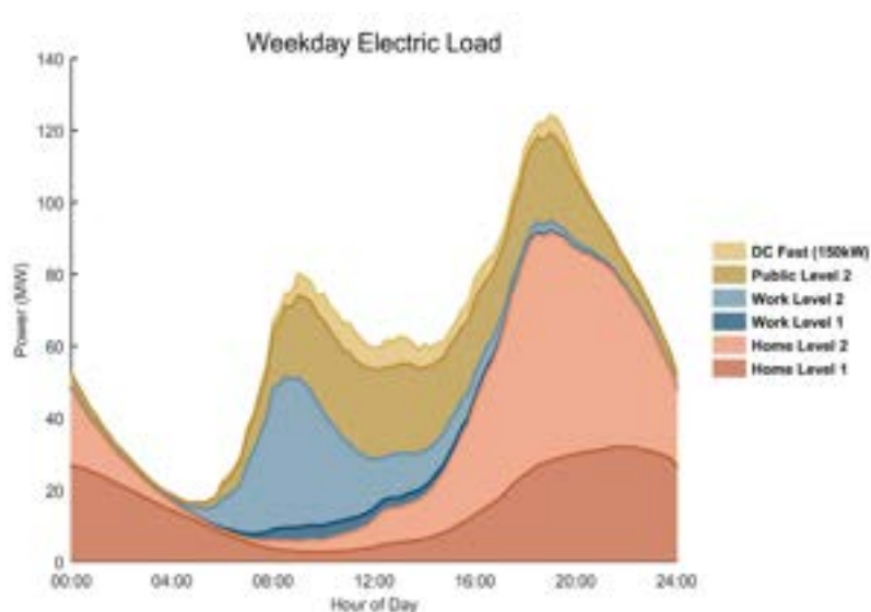
Load Forecasts for Milwaukee under an Aggressive Adoption Scenario
