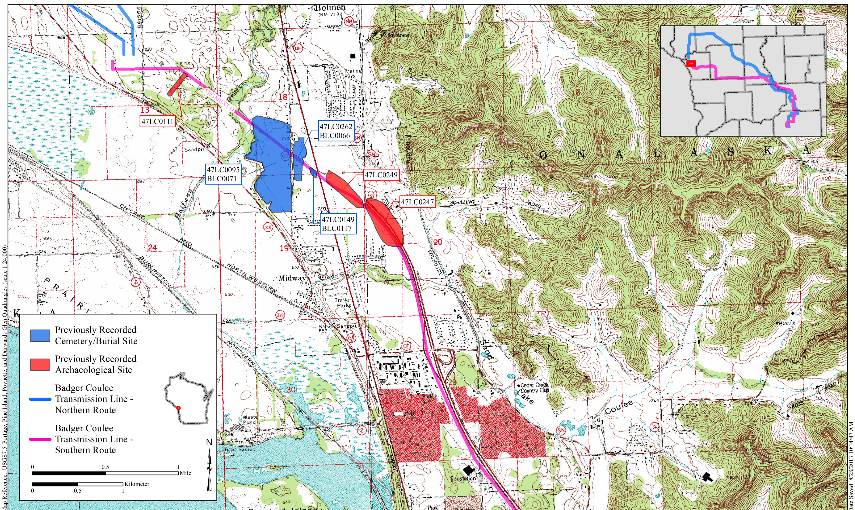
Figure 2.2.10-2a. Badger Coulee Transmission Line and Locations of Previously Recorded Archaeological and Cemetery/Burial Sites within Segment O
