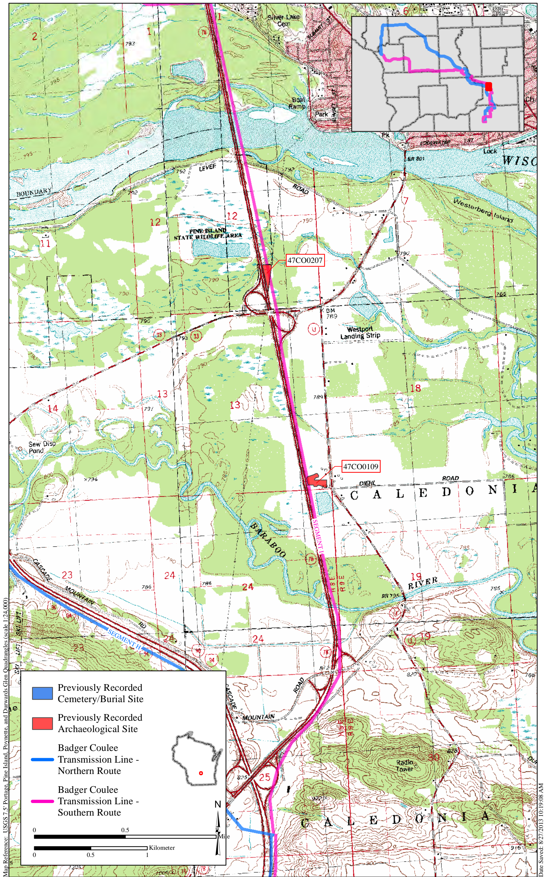
Figure 2.2.6-1c. Badger Coulee Transmission Line and Locations of Previously Recorded Archaeological and Cemetery/Burial Sites within Segment I
